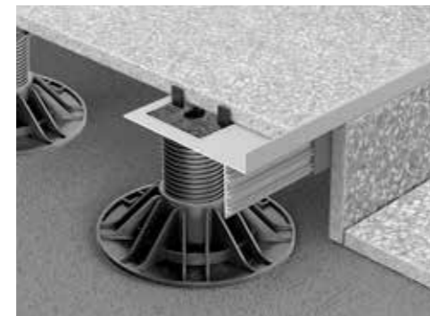
PROSUPPORT PROFILE T - VARNISHED ALUMINIUM bar length 2,7 lm - pack. 20 Pcs - 54 lm
