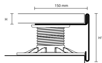
TOP PROFILE PROSUPPORT B - VARNISHED ALUMINIUM length 2,7 lm
